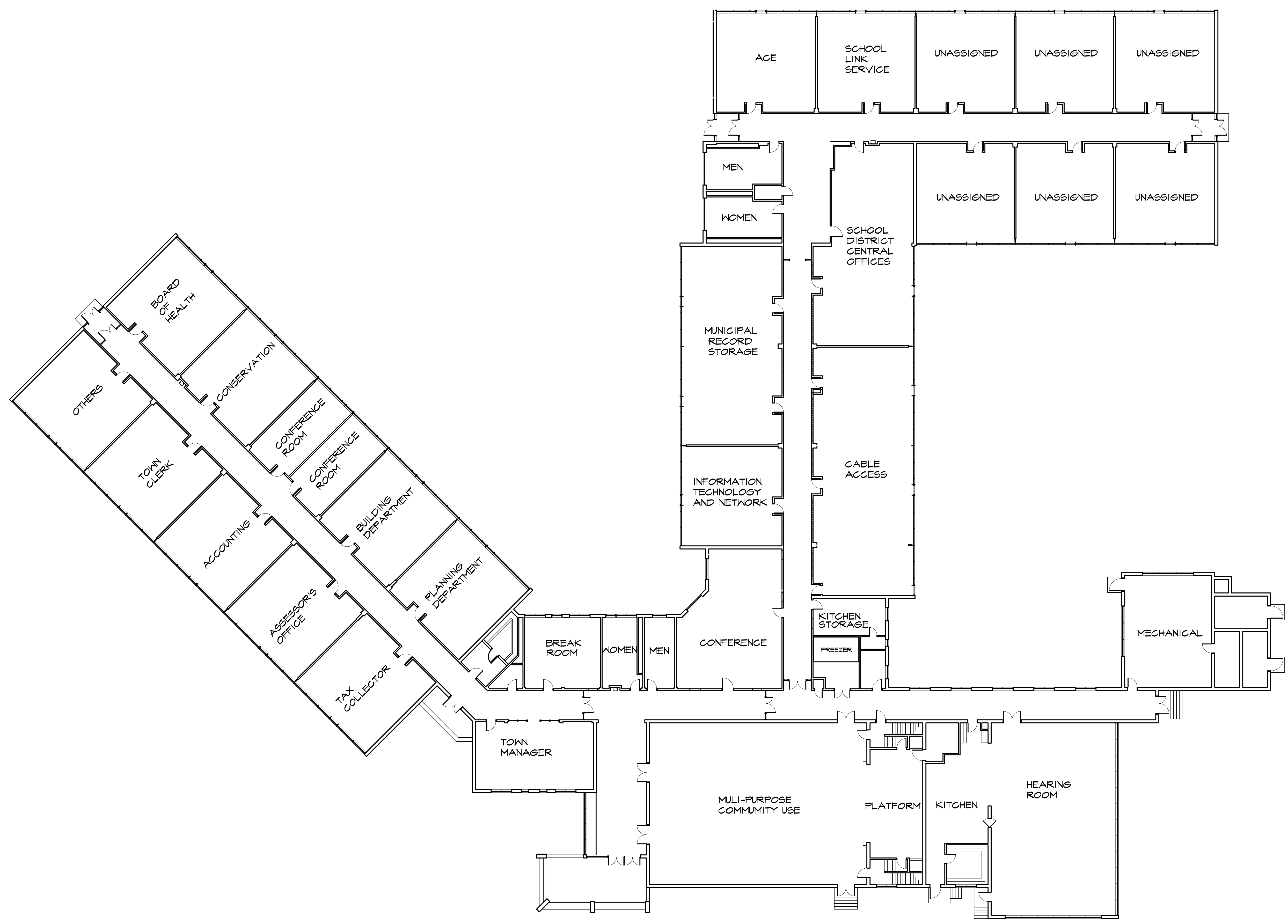
FLOOR PLAN: FIRST FLOOR 1/16" = 1'-0"
